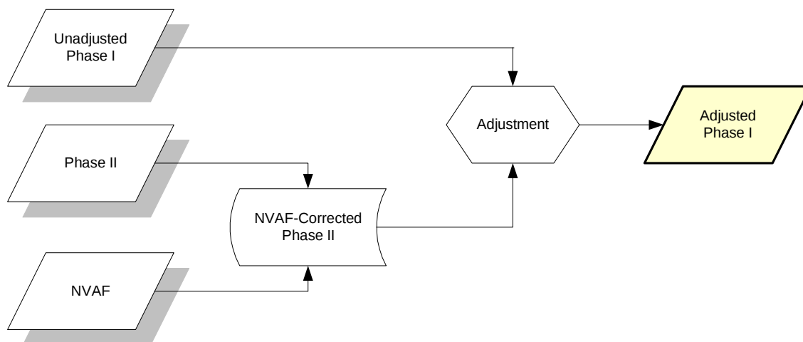
Figure 1. VRI flow-chart.
