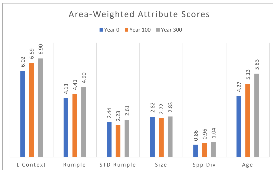
Figure 25. Current (Year 0) ecosystem integrity attribute scores compared with modelled attribute scoring for years 100 and 300 for all study areas combined. L CONTEXT = landscape context score; RUMPLE = mean rumple score; SD RUMPLE = standard deviation of rumple score; SIZE = size score; SPP DIV = species diversity score; AGE = stand age score.
