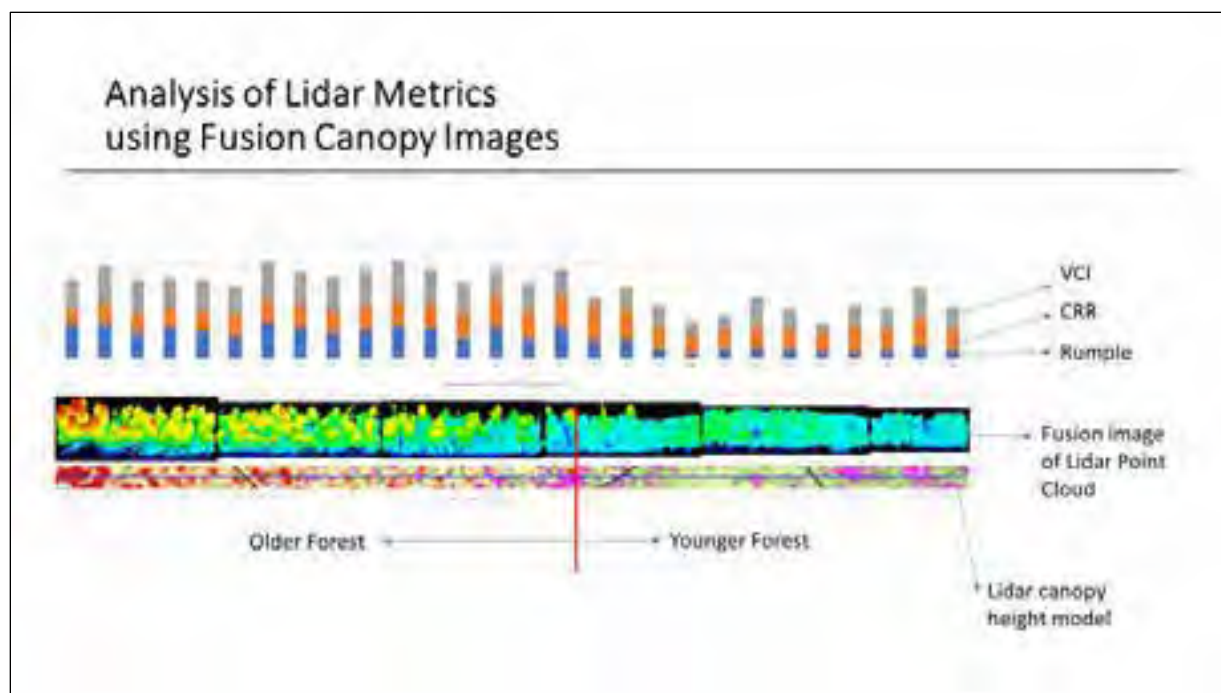
Figure 1. Example of lidar sample transect, TFL 37. Stacked graphs of three lidar metrics are shown above the Fusion lidar point cloud canopy images. VCI = vertical canopy index; CRR = canopy relief ratio; see text for further explanation.
